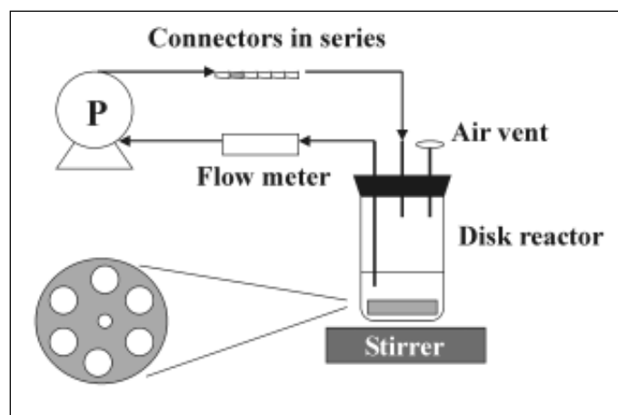
Figure 2. Biofilm disk reactor system.
